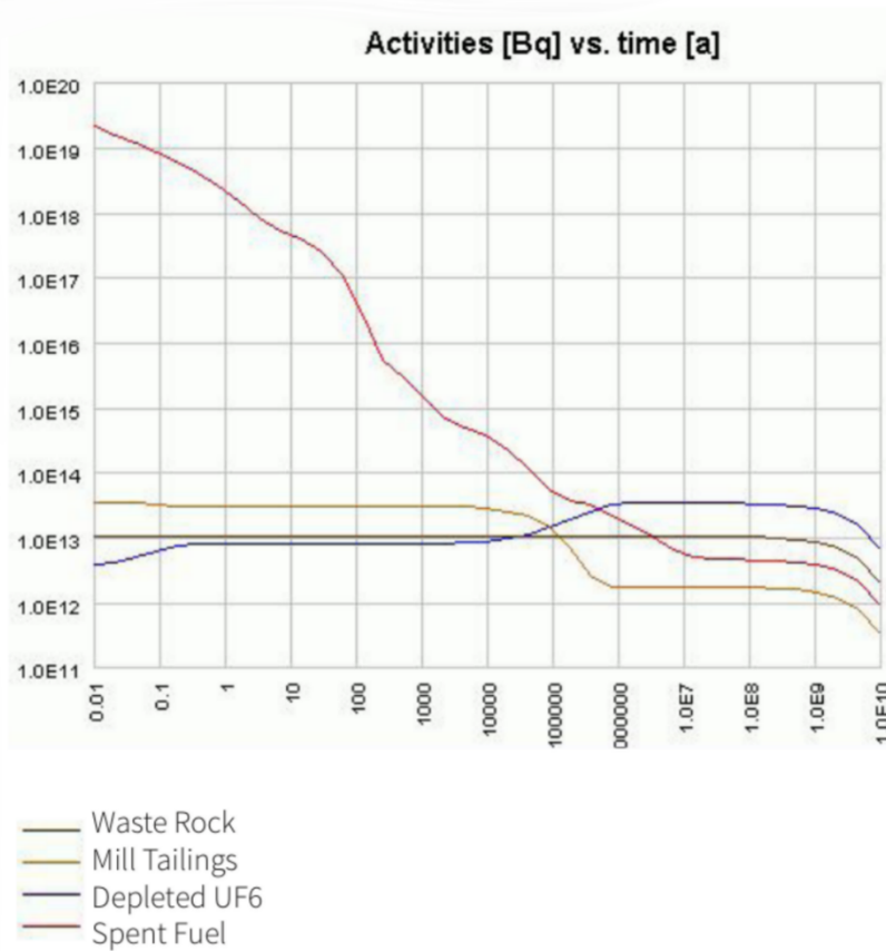
Figure 1: Example of decay of spent nuclear fuel generated by a 1 000 MW nuclear power reactor each year 47
