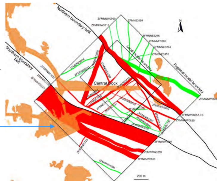
Figure 1-4. Ground-surface intersection of deformation zone traces (Curtis et al. 2010). Coloured by confidence in existence: high = red, medium = green.
